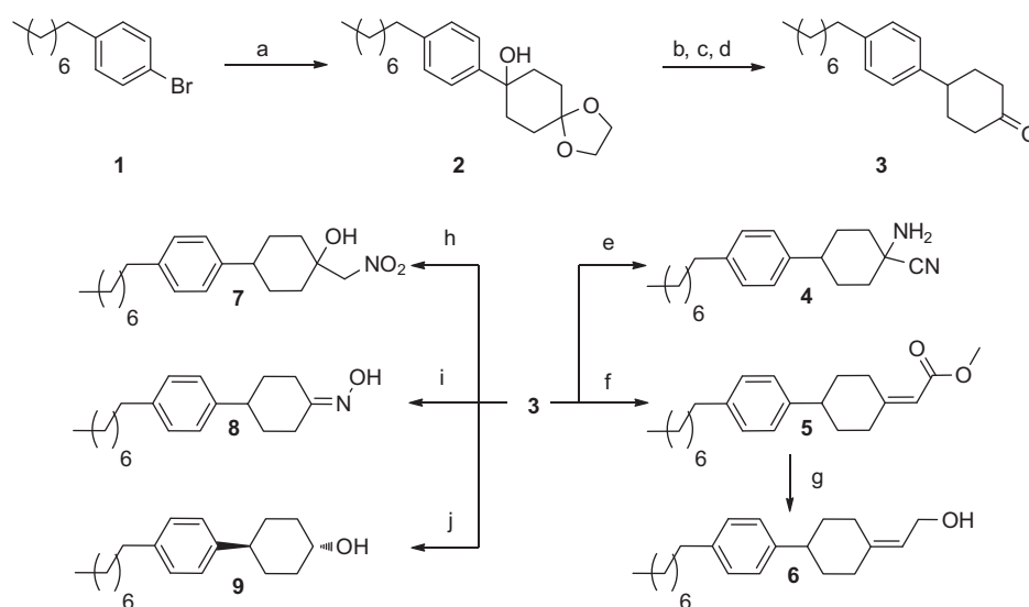
Scheme 1. Reagents and conditions: (a) n -BuLi, -78^{\circ}\text{C} , THF, then 1,4-cyclohexanedione monoketal, 2 h, 75%; (b) TsOH, toluene, 65^{\circ}\text{C} , 1 h; (c) \text{H}_2 , Pd/C, EtOH, 20 h; (d) AcOH/ \text{H}_2\text{O} (3:1), 65^{\circ}\text{C} , 2 h, 76% over 3 steps; (e) KCN, \text{NH}_4\text{Cl} , MeOH, reflux, 23%; (f) \text{NaO}^t\text{Bu} , methyl diethylphosphonoacetate, \text{CH}_2\text{Cl}_2 , -78^{\circ}\text{C} to rt, 82%; (g) DIBAL-H (1 M in toluene), \text{CH}_2\text{Cl}_2 , 0^{\circ}\text{C} to rt, 79%; (h) \text{CH}_3\text{NO}_2 , NaOEt, EtOH, 0^{\circ}\text{C} to rt, 62%; (i) hydroxylamine hydrochloride, pyridine, 80^{\circ}\text{C} , 83%; (j) \text{NaBH}_4 , MeOH, rt, 12 h, 72%.
