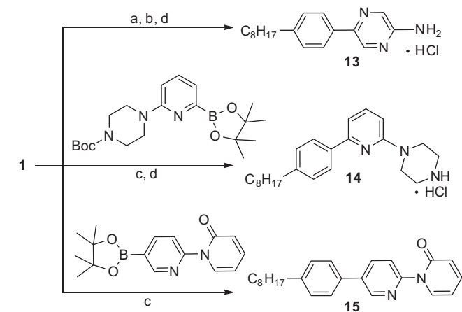
Scheme 3. Reagents and conditions: (a) n -BuLi, –78 °C, THF, 15 min, then B(OMe) 3 , rt, 1 h, then 10% aq. HCl, 58%; (b) 5-Bromo-2-pyrazineamine, Pd(OAc) 2 , K 2 CO 3 , SPhos, CH 3 CN/H 2 O (1:1.5), reflux, 6 h, 72%; (c) Pd(OAc) 2 , K 2 CO 3 , SPhos, CH 3 CN/H 2 O (1:1.5 equiv), reflux, 12 h, 81–92%; (d) HCl (g), THF, 1 min., 92–95%.
