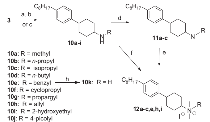
Scheme 2. (a) R-NH 2 , NaBH(OAc) 3 , CH 2 Cl 2 , rt, 2 h, 63–77%; (b) R-NH 2 , NaBH 3 CN, MeOH, 0 °C to rt, 12 h, 64–82%; (c) R-NH 2 , LiBH 4 , –78 °C to rt, 20 h, 73–82%; (d) (CH 2 O) n , HCOOH, MeOH, reflux, 6 h, 66–93%; (e) MeI, CH 3 CN, reflux, 2 h, 68–72%; (f) MeI, K 2 CO 3 , CH 3 CN, reflux, 2 h, 39–73%; (h) H 2 , 10% Pd/C, MeOH, 84%.
